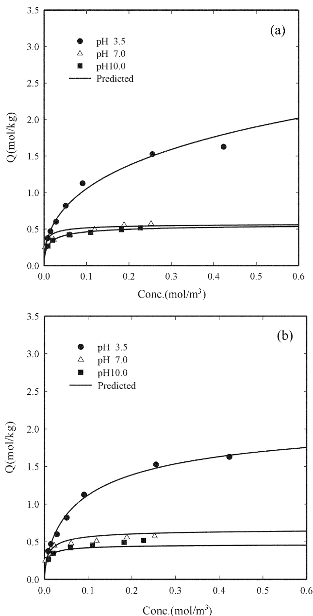
Fig. 4. Experimental data and predicted adsorption isotherms for 2,4-DNP-F400 system for different initial pH at 298.15 K (a: Sips Eq., b: pH dependent Sips Eq.).
